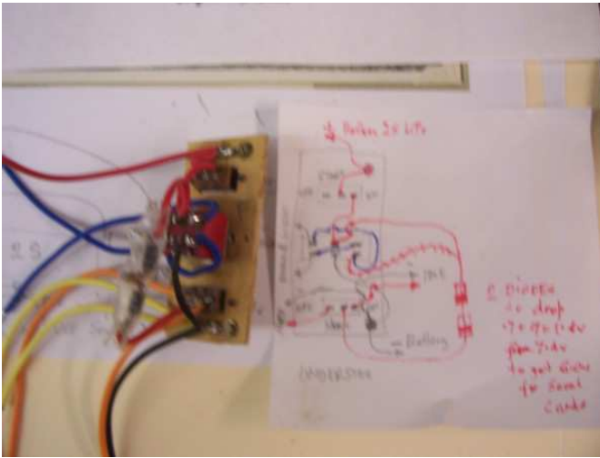
Switch arrangement & wiring diagram.
