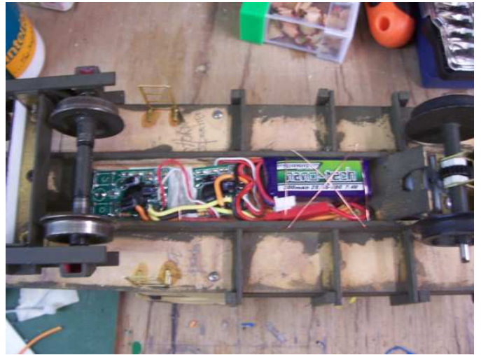
Two 20 second sound cards & 2S 300mAh LiPo.
